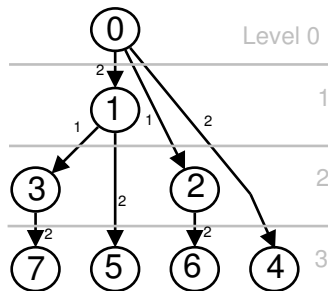
Fig. 10. Binomial tree pattern with 8 processes annotated with the maximum congestion along each path.
