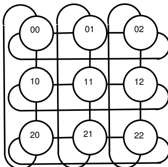
Fig. 14. 3-ary 2-cube network with endpoint numbering.
