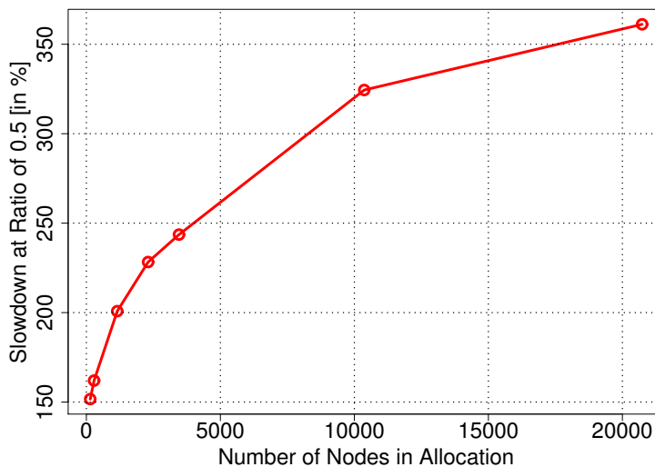
Fig. 13. Slowdown with increasing communicator size and a fixed perturbation ratio of 1/2 .
