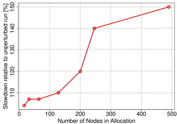
Fig. 5. Slowdown of an allreduction operation with increasing allocation size and a fixed perturbation ratio of 1/2 on an InfiniBand fat-tree with full bisection bandwidth.
