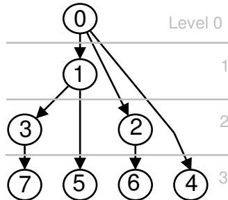
Fig. 7. Binomial tree pattern among 8 processes.
