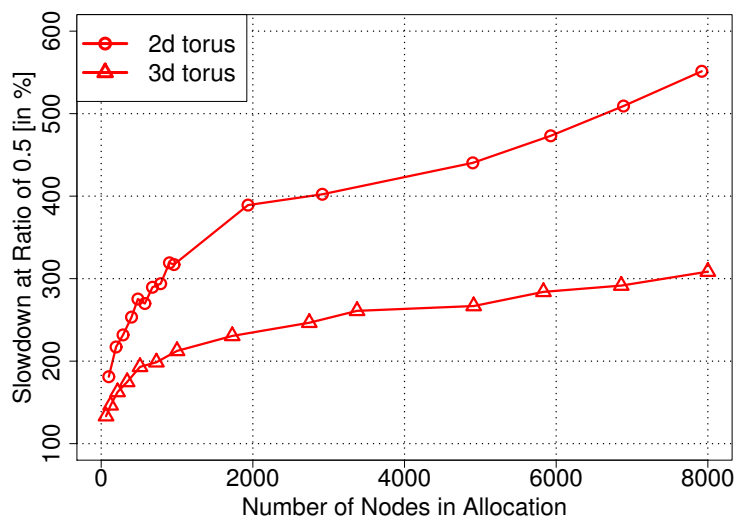
Fig. 16. The influence of background communication on k -ary 2-cubes and k -ary 3-cubes of different sizes and perturbation ratio 1/2 .
