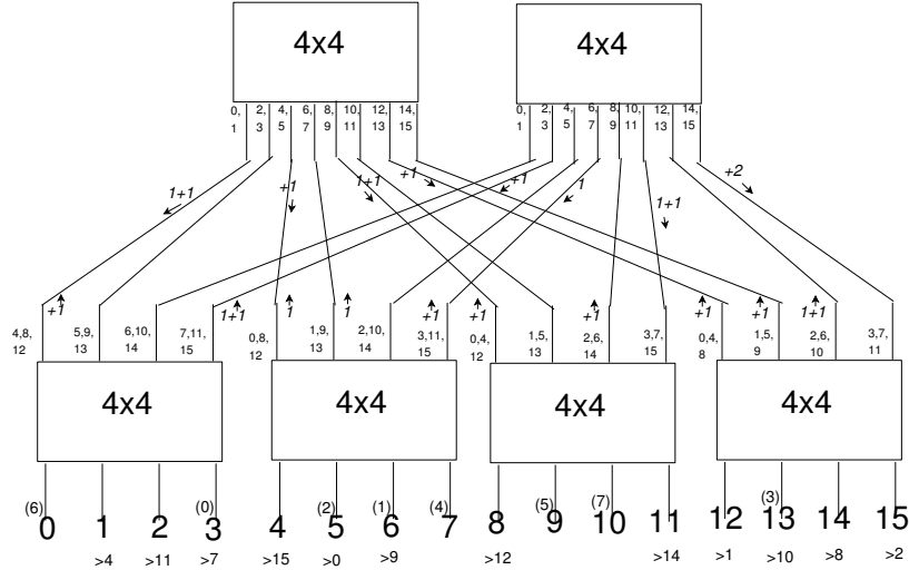
Fig. 9. Schematic example of Figure 8 with perturbation communication prefixed with "+" at the links. Communication peers are indicated with >.
