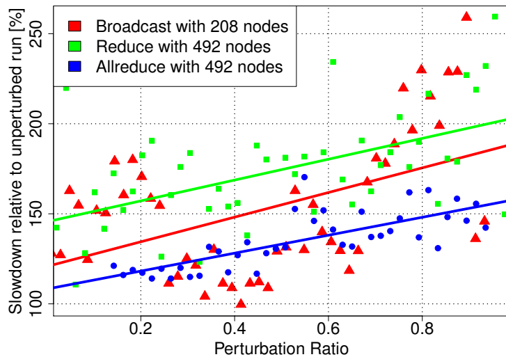
Fig. 4. Average slowdown due to network noise for fixed allocations with different perturbation ratios on an InfiniBand fat-tree.
