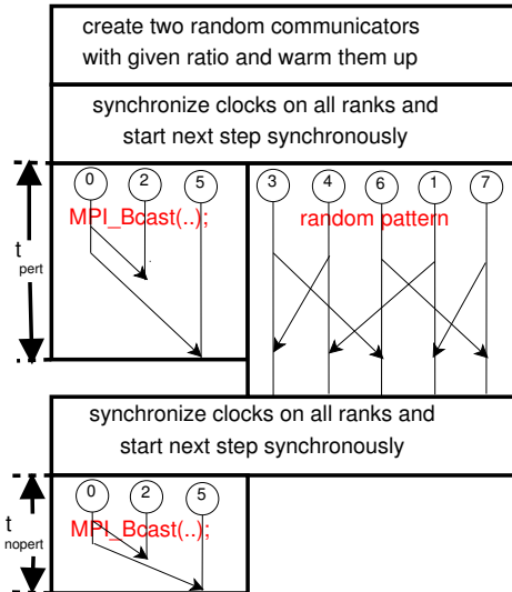
Fig. 2. One round of the used benchmarking scheme on 8 processes and a perturbation ratio of 5/8=0.625 . Two process-disjoint communicators perform perturbation and collective communication, respectively.
