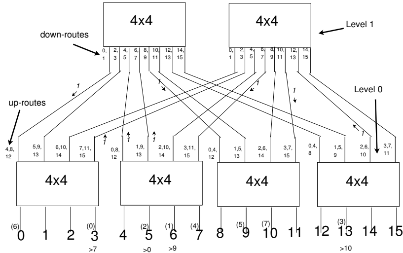
Fig. 8. Schematic example network with 8 processes performing the third level of a binomial broadcast on 8 processes. Processes are mapped randomly to nodes and process numbers are indicated in brackets (e.g., process 6 runs on node 0). Communication peers are prefixed with > and occupied links are indicated with arrows and the number of messages using the link. Each link is annotated with the targets that it routes to.
