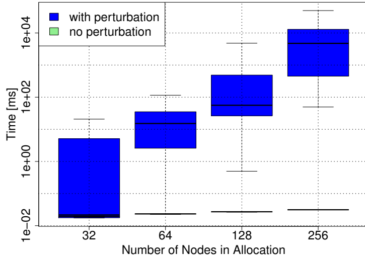
Fig. 6. Boxplot of the collective latencies with background noise and a perturbation ratio of 1/2 on the three-dimensional torus network of a BlueGene/P.
