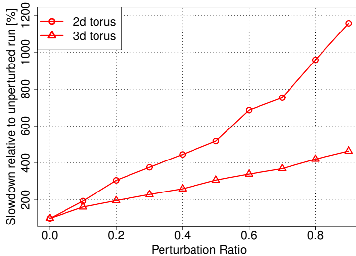
Fig. 15. The slowdown for 100-ary 2-cube and 20-ary 3-cube executing a binomial tree pattern.
